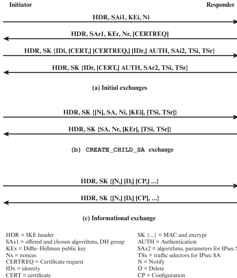
Figure 9.11 IKEv2 Exchanges
