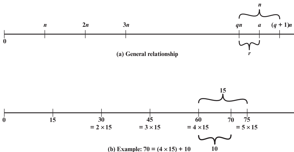
Figure A.1 The Relationship a = qn + r ; 0 \leq r < n
